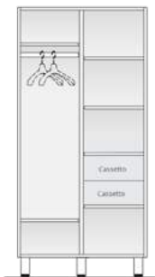
Cod. ADR635 Arm. a 2 ante, 2 cas. e 5 rip. L900 x P560 x H1910 mm
